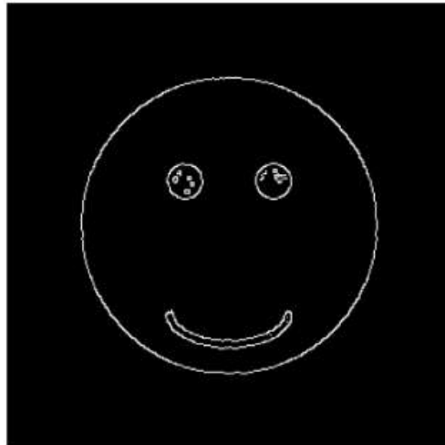
Mid-Level: Features
